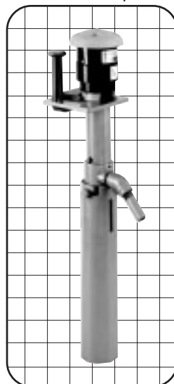
Trash Trap
